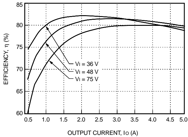
Figure 6. LW025A Typical Converter Efficiency vs. Output Current
