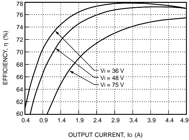
Figure 5. LW025F Typical Converter Efficiency vs. Output Current
